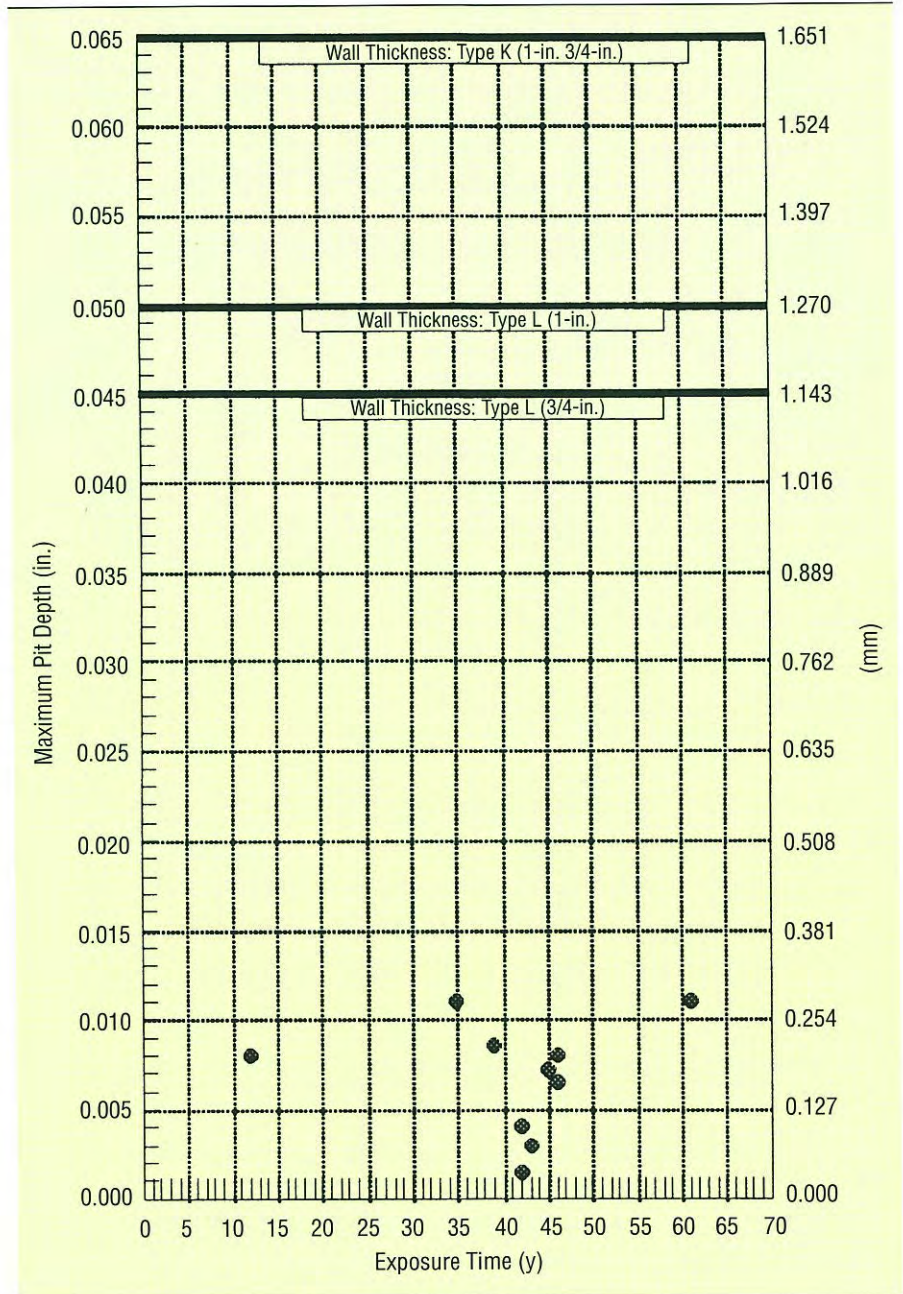
FIGURE 2 Maximum pit depth as a function of exposure time to the various soil conditions (points). Dark horizontal lines represent the original pipe wall thicknesses.
