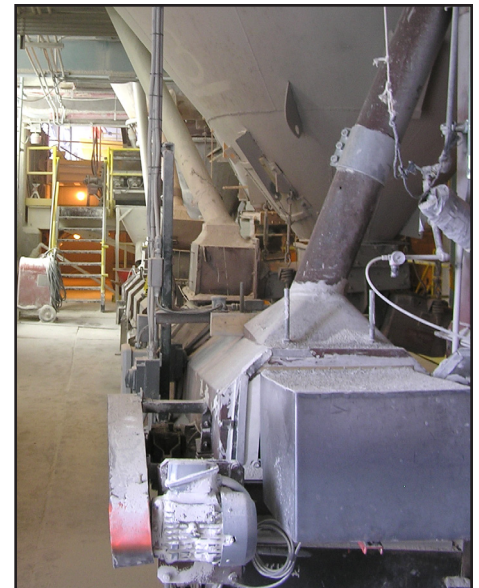
Figure 3. A 2-hp SE&A IEEE Plus belt conveyor motor (lower right of photo) that transports finely-ground product to the beneficiation department. It was one of the first copper-rotor motors installed during the current replacement program. The data plate lists the motor's NEMA nominal efficiency at 87.5%, one full percentage point higher than called for under NEMA Premium standards.
